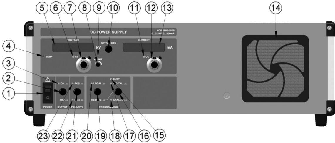
Front view with controls
